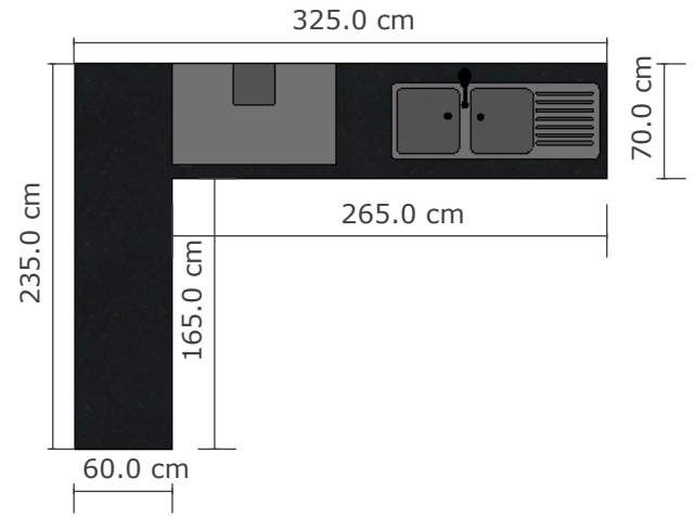
I :: A10 wet kitchen 002 scale: 1 : 20 (top view)
