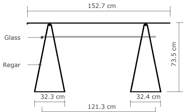
D :: B4 Desk Table 001 scale: 1 : 20 (front view)
