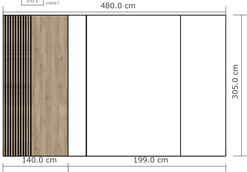
K :: B11 TV backdrop 001 scale: 1 : 50 (Front view)
