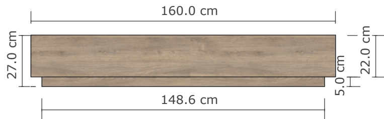
R :: A19 Divan + drawer 001 scale: 1 : 20 (front view)
