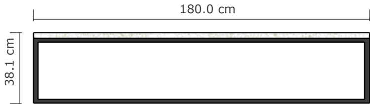
C :: A3CONSOLE TABLE 001 scale: 1 : 20 (front view)
