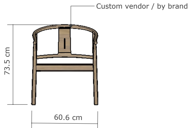
V :: B22 working chair 001 scale: 1 : 50 (Front view)
