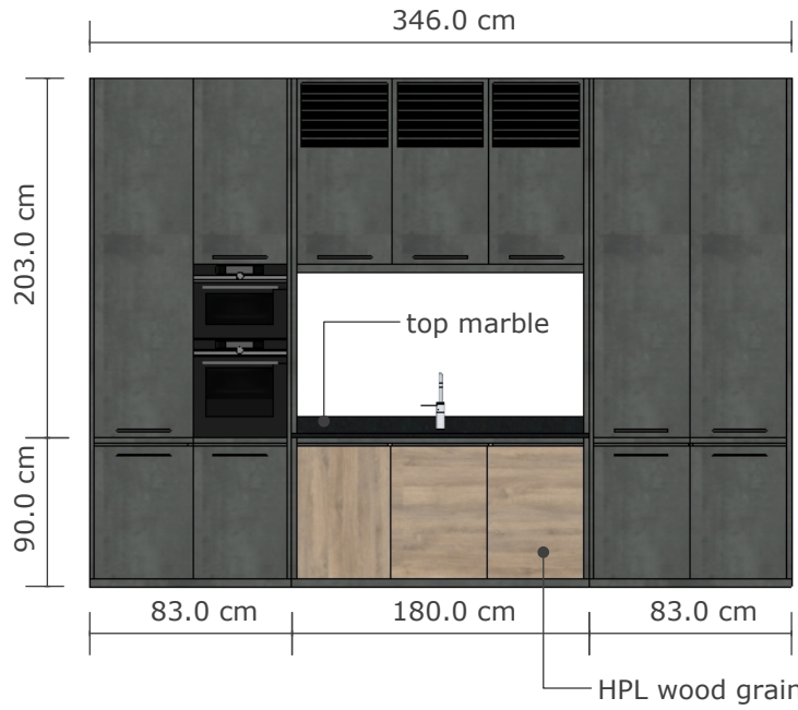
I :: A9 kitchen counter & upper 001 scale: 1 : 20 (front view)
