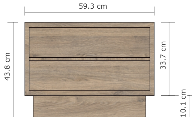
V :: A24 Bedside cabinet 001 scale: 1 : 20 (front view)
