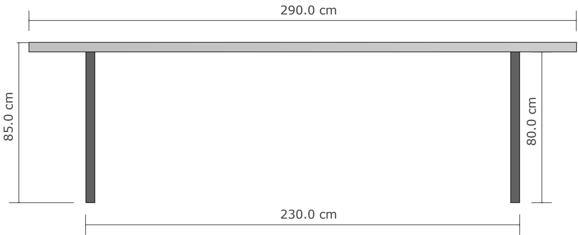
D :: A4 meeting table 001 scale: 1 : 20 (front view)
