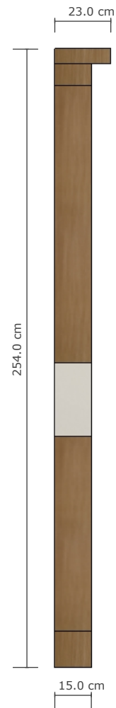
A :: PARTISI 002 tampak samping
