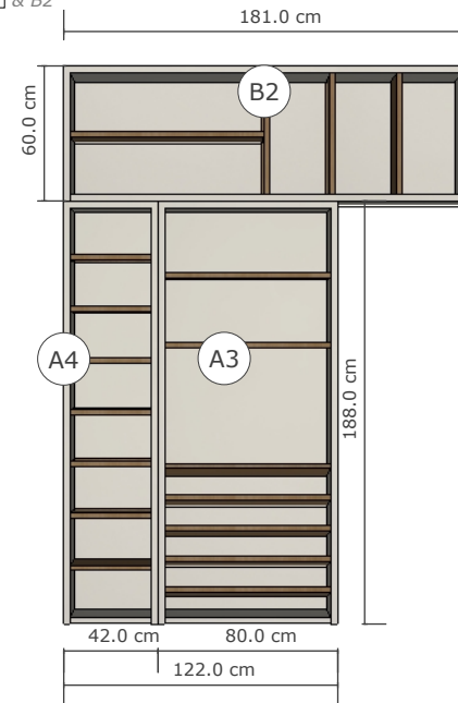
A :: WALK IN CLOSET 002 tampak depan A3, A4, & B2
