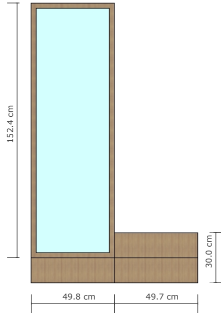
A :: STANDING MIRROR 004 tampak depan
